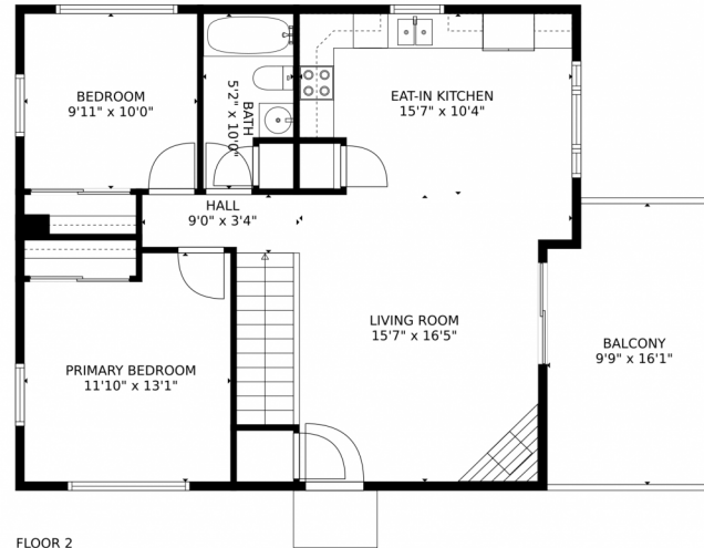
FLOOR 2
