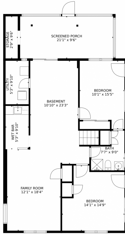
FLOOR 1
