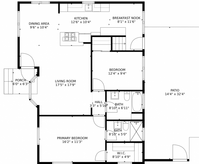
FLOOR 2
