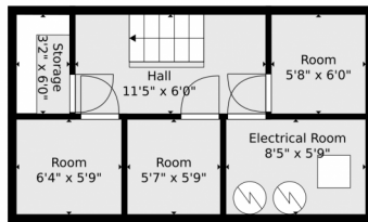
Floor 1
