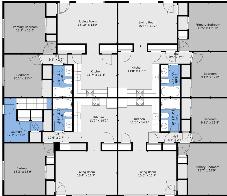
Floor 2
