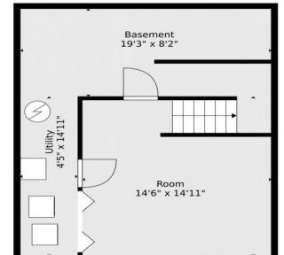
floorplan_single_0
