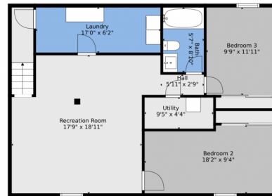
Floor 1
