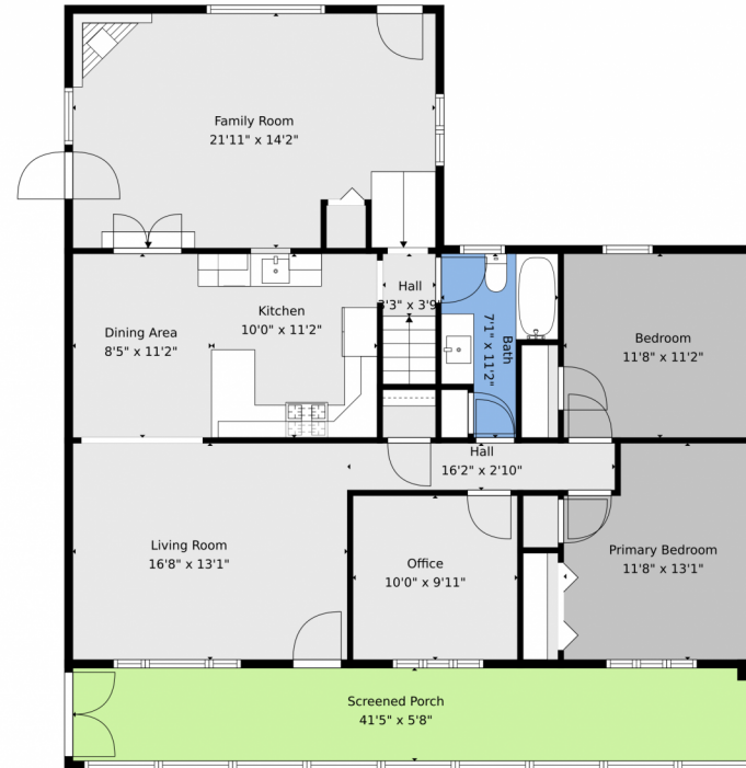
1st Floor
