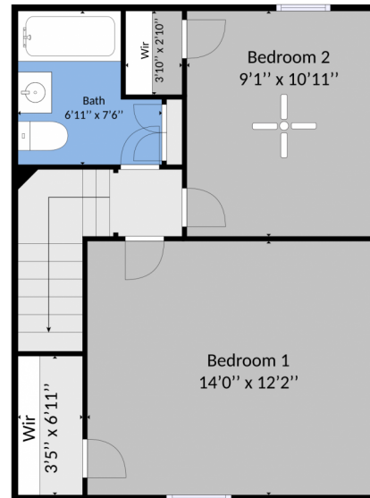
2nd Floor
